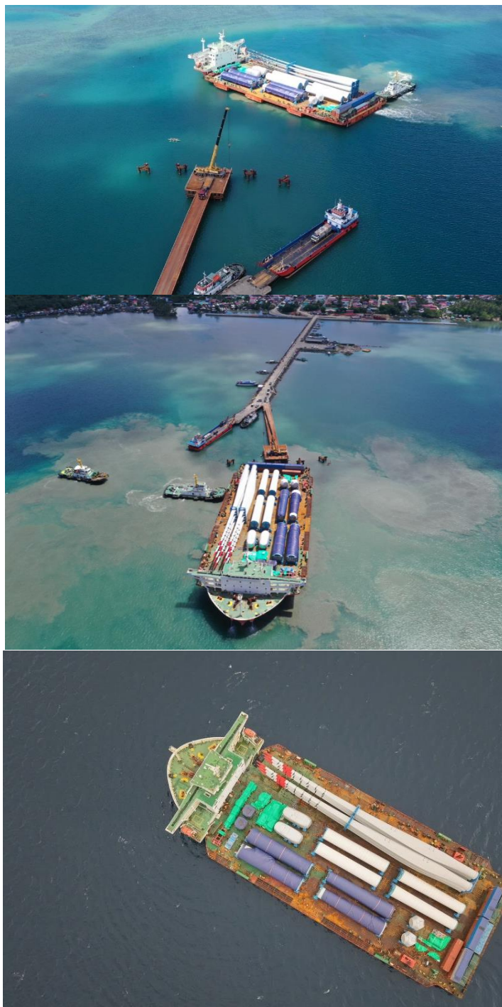
First Delivery of Wind Turbine Components at Alternergy's jetty on Alabat Island, Quezon Province
